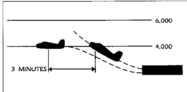
FIG 6-2-8 Minima on Same Course
