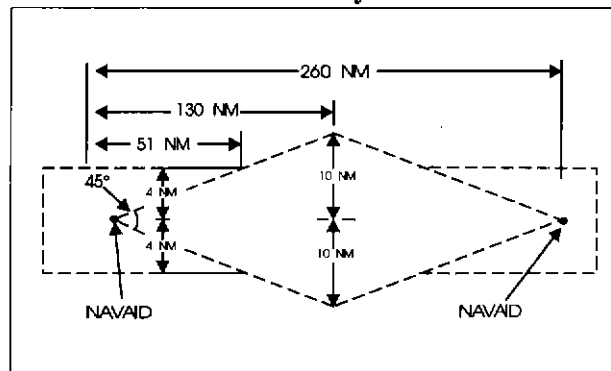
FIG 6-5-4 Minima Along Other Than Established Airways or Routes
