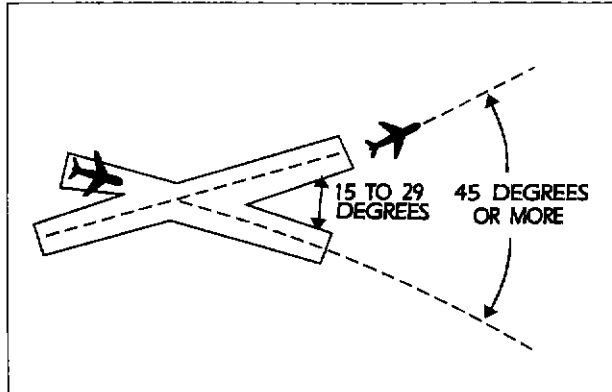
FIG 6-2-7 Minima on Diverging Courses
