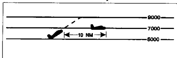
FIG 6-4-8 Climbing Through Another Aircraft's Altitude DME Separation
