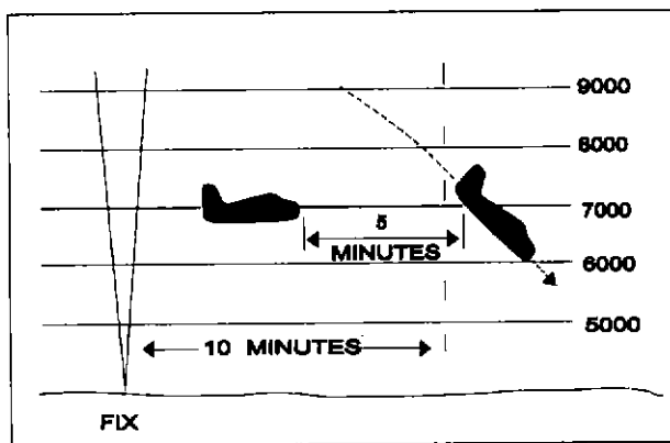
FIG 6-4-9 Descending Through Another Aircraft's Altitude Timed Separation
