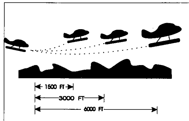
FIG 3-12-6 Sea Lane Arrival Operations
