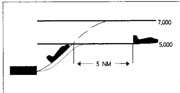
FIG 6-2-9 Minima on Same Course
