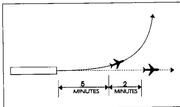
FIG 6-2-2 Minima on Diverging Courses
