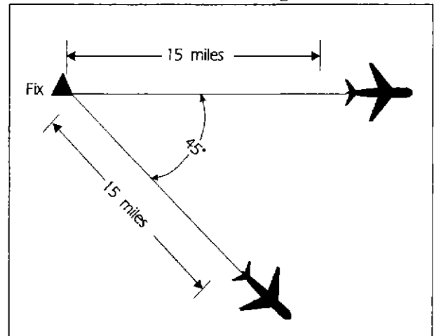
FIG 8-4-13 Track Separation Dead Reckoning
