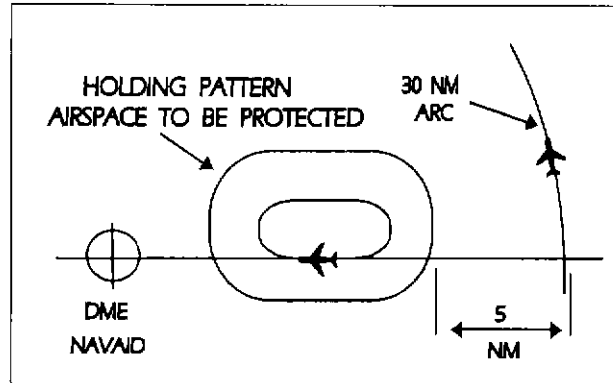
FIG 6-5-3 DME Arc Minima
