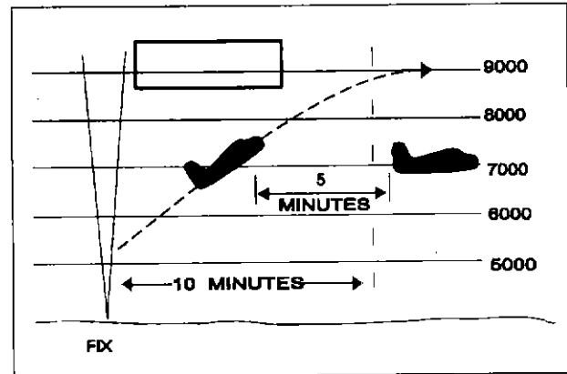
FIG 6-4-10 Climbing Through Another Aircraft's Altitude Timed Separation
