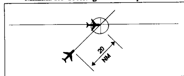
FIG 6-4-12 Minima for Crossing Courses Separation
