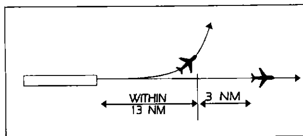
FIG 6-2-3 Minima on Diverging Courses
