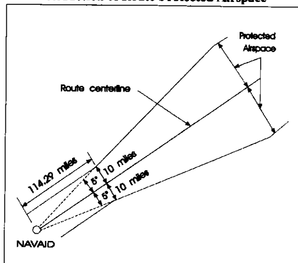
FIG 8-4-9 Reduction of Route Protected Airspace
