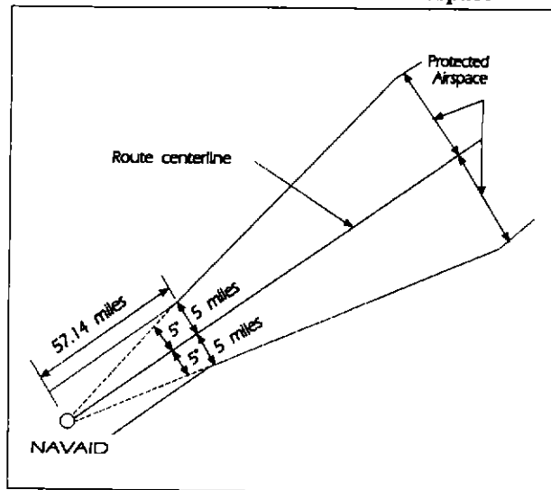
FIG 8-4-8 Reduction of Route Protected Airspace
