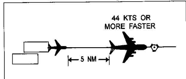
FIG 6-4-1 Minima on Same Course 44 Knots or More Separation
