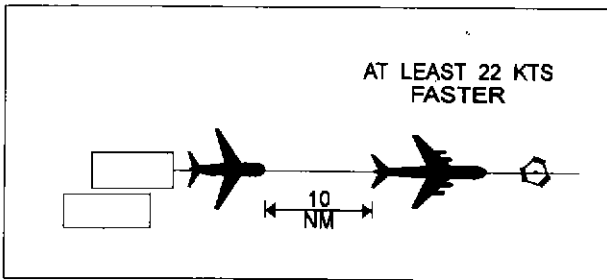
FIG 6-4-4 Minima on Same Course 22 Knots or More Separation
