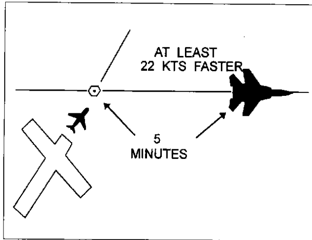
FIG 6-4-6 Minima on Crossing Courses 22 Knots or More Separation
