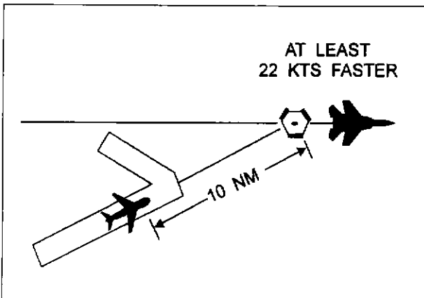
FIG 6-4-5 Minima on Converging Courses 22 Knots or More Separation
