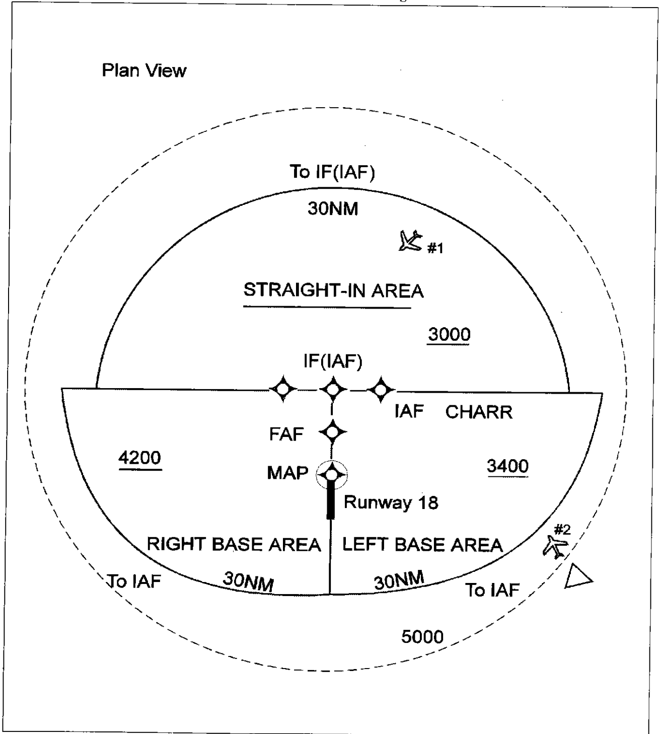
FIG 4-8-2 Basic "T" and TAA Design
